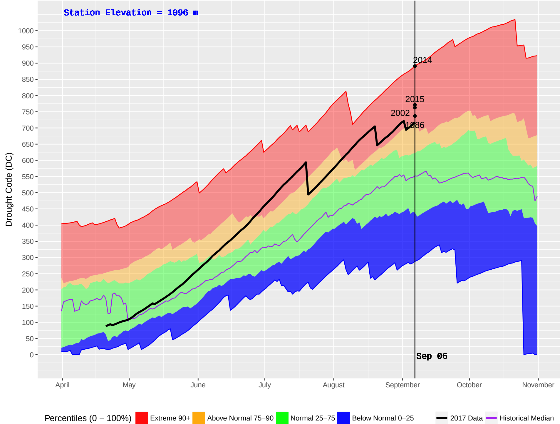
ANAHIM LAKE HUB (213) : Historical (1981–2016) and Current (2017) Noon Drought Code (DC)
