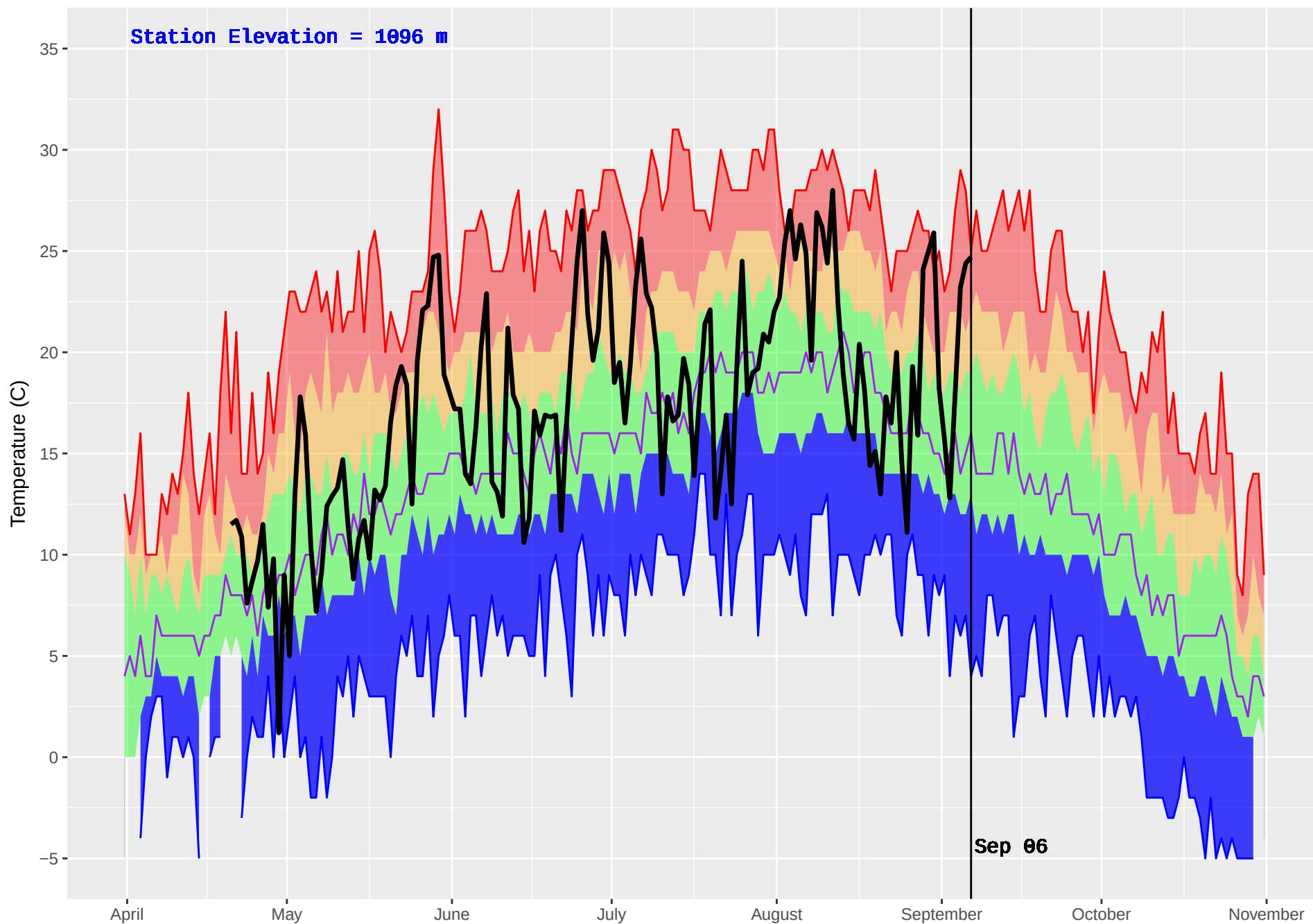
ANAHIM LAKE HUB (213) : Historical (1981–2016) and Current (2017) Noon Temperature
